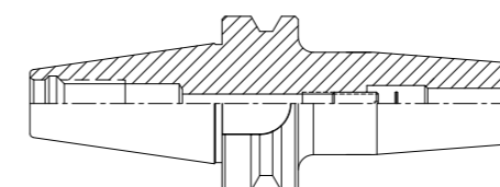
热胀刀柄 Shrink Fit Chuck
